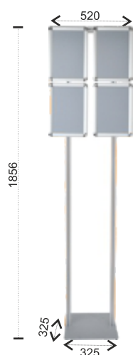
SST-PMA441V SST-PMA442V
